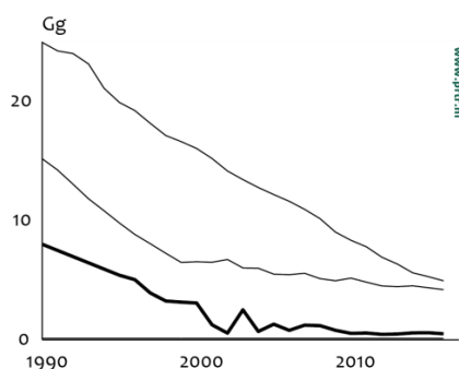
Figure 2.5 PM 2.5 emission trends 1990-2015
